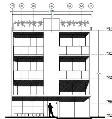
FACHADA PRINCIPAL
